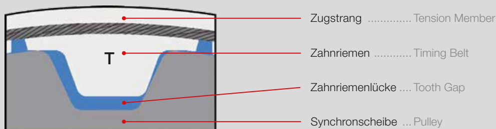
Normale Lückenform Normal Backlash Tooth Gap
