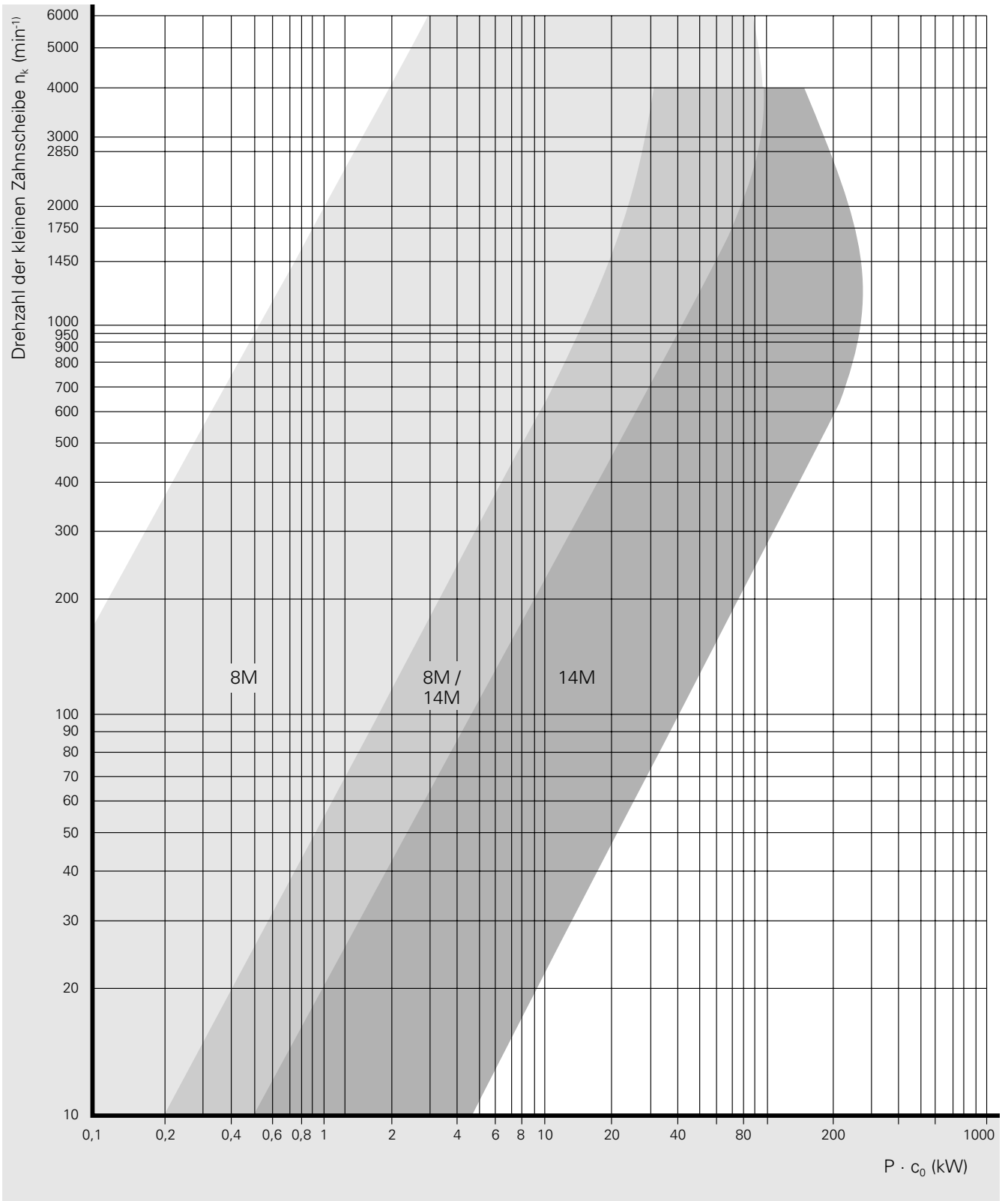
CONTI SYNCHROBELT® HTD Zahnriemen 8M, 14M
