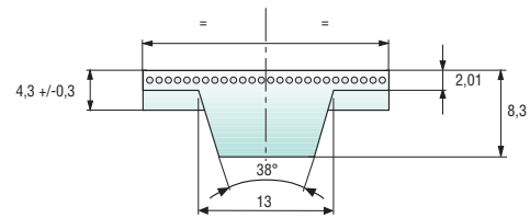
notched guide
